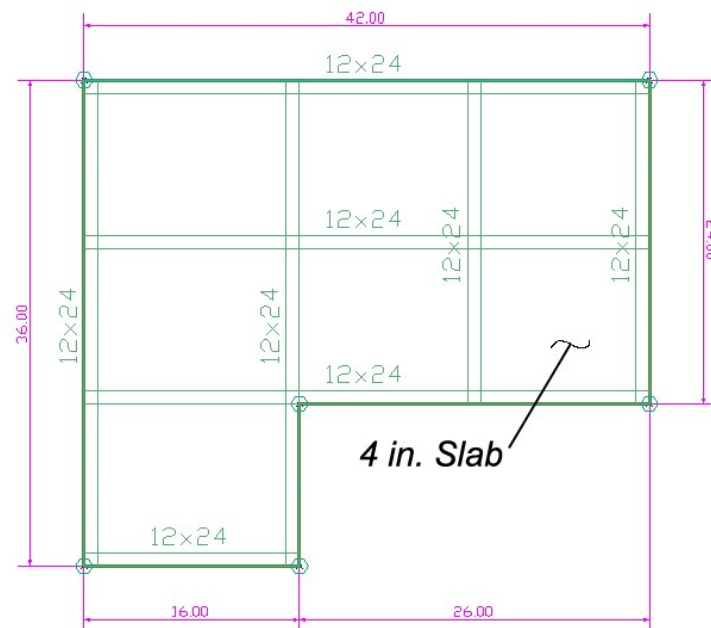
FIGURE B4.1-1 - PLAN OF SLAB USED FOR DESIGN
