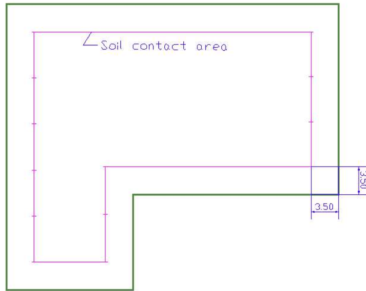
FIGURE B4.5.2-1 PLAN OF SLAB SHOWING “a” = 3.5 FT FOR CENTER LIFT CONDITION
