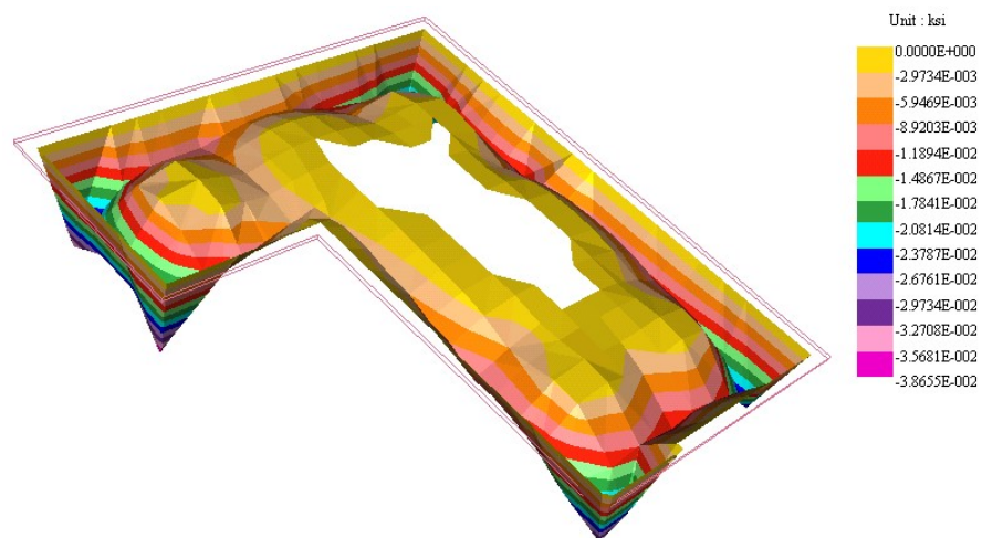
FIGURE B4.5.2-10 - DISTRIBUTION OF SOIL PRESSURE
