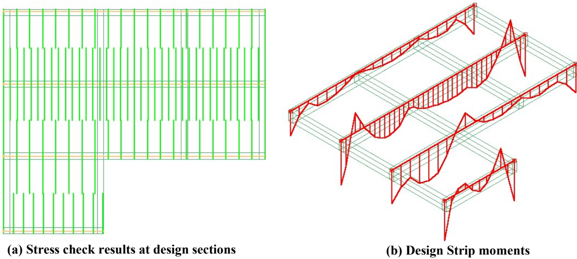
FIGURE B4.5.3-5 - STRESS CHECK AND DESIGN MOMENTS FOR DESIGN STRIPS IN THE LONG DIRECTION UNDER EDGE LIFT CONDITION
