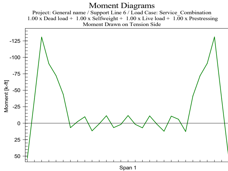
FIGURE B5.2.1-3 - DISTRIBUTION OF MOMENT FOR DESIGN STRIP 6
