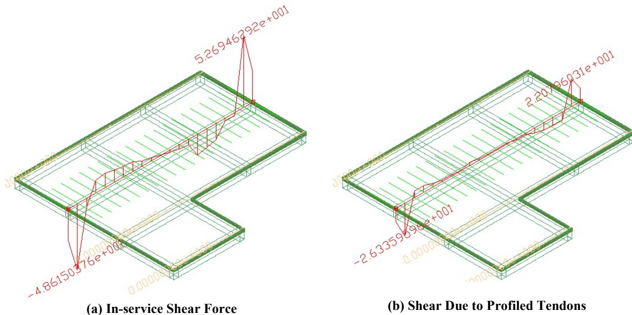
FIGURE B4.5.2-8 - DISTRIBUTION OF SHEAR AT GRIDLINE 2
