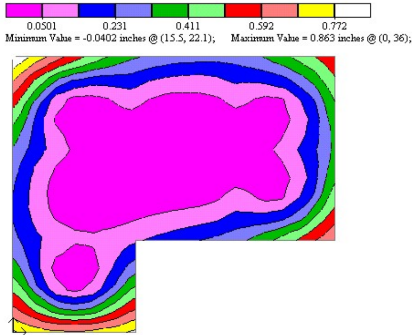
FIGURE B4.5.2-3 DEFLECTION CONTOUR OF SLAB FOR CENTER LIFT CONDITION
