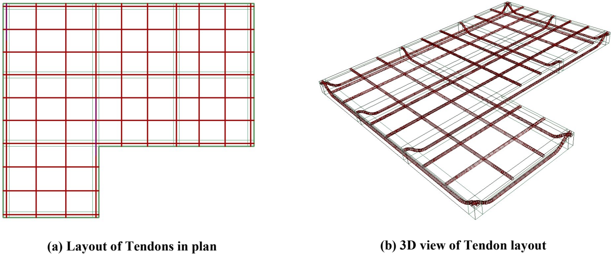
FIGURE B4.2-1 TENDON LAYOUT
