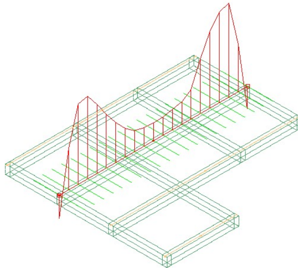
FIGURE B4.5.2-5 - DESIGN STRIP AND BENDING MOMENT AT LINE 2 (The green lines are the design sections at which the plotted moment distribution is calculated.)
