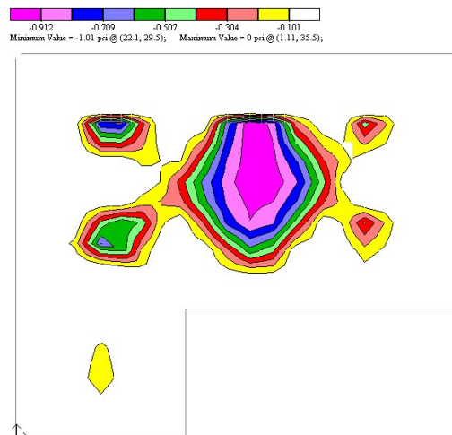
FIGURE B4.5.3-3 - DISTRIBUTION OF SOIL PRESSURE FOR EDGE LIFT EQUAL TO 0.05"
