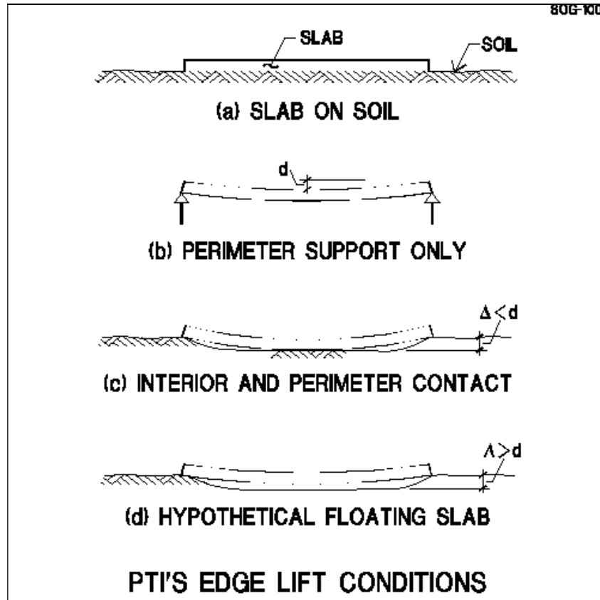
FIGURE B5.2.9-1 - PTI'S EDGE LIFT CONDITIONS
