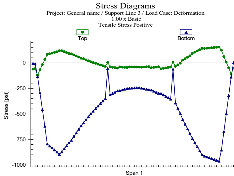
FIGURE B4.5.2-6 - TOP AND BOTTOM FIBER DESIGN STRESSES AT GRIDLINE 2
