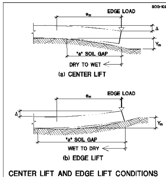
FIGURE B1.3-1 CENTER LIFT AND EDGE LIFT CONDITIONS
