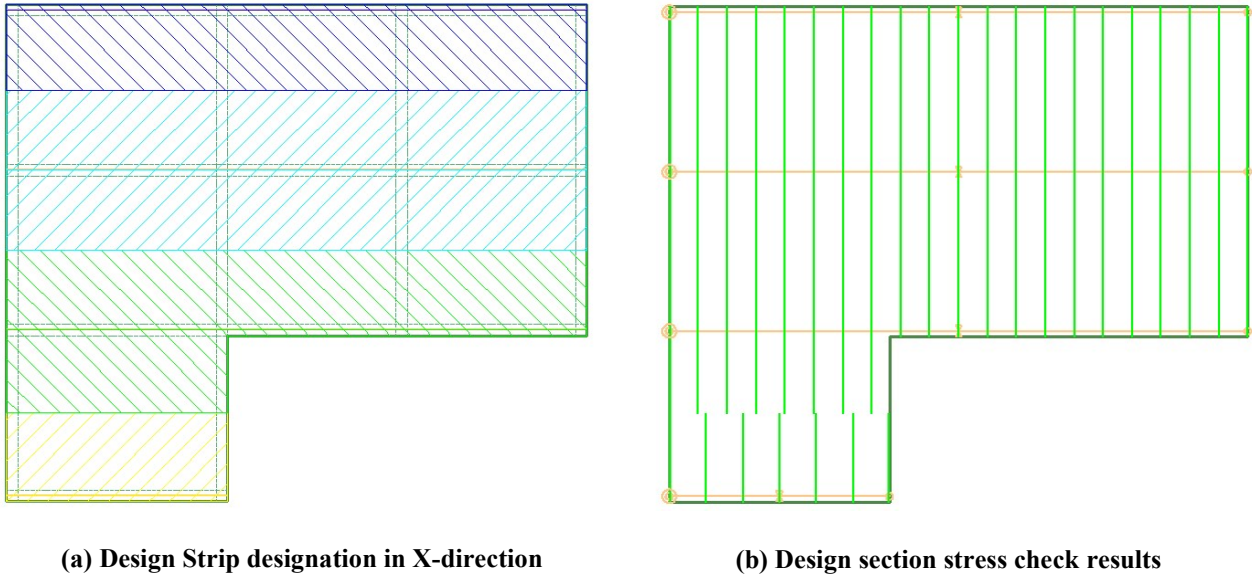
FIGURE B4.5.2-4 - DESIGN STRIPS AND STRESS CHECK RESULTS IN THE X-DIRECTION FOR CENTER LIFT CONDITION
