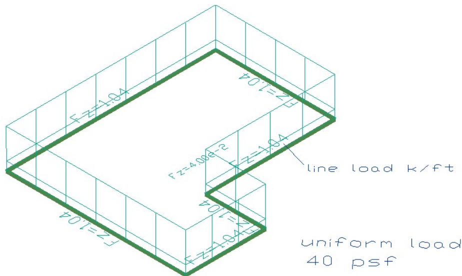
FIGURE B4.4-1 VIEW OF SPECIFIED LOADING
