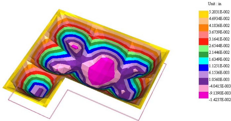
FIGURE B4.5.3-4 - DEFLECTION OF SLAB FOR EDGE LIFT EQUAL TO 0.05"
