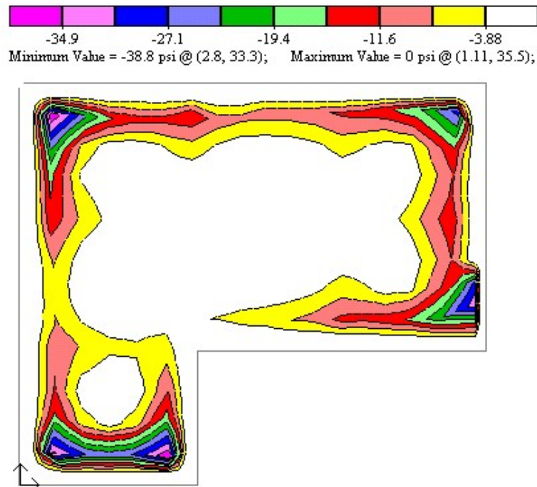
FIGURE B4.5.2-9 - DISTRIBUTION OF SOIL PRESSURE FOR CENTER LIFT CONDITION
