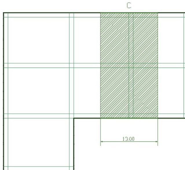
FIGURE B4.5.3-1 - PLAN OF SLAB SHOWING THE DESIGN STRIP
