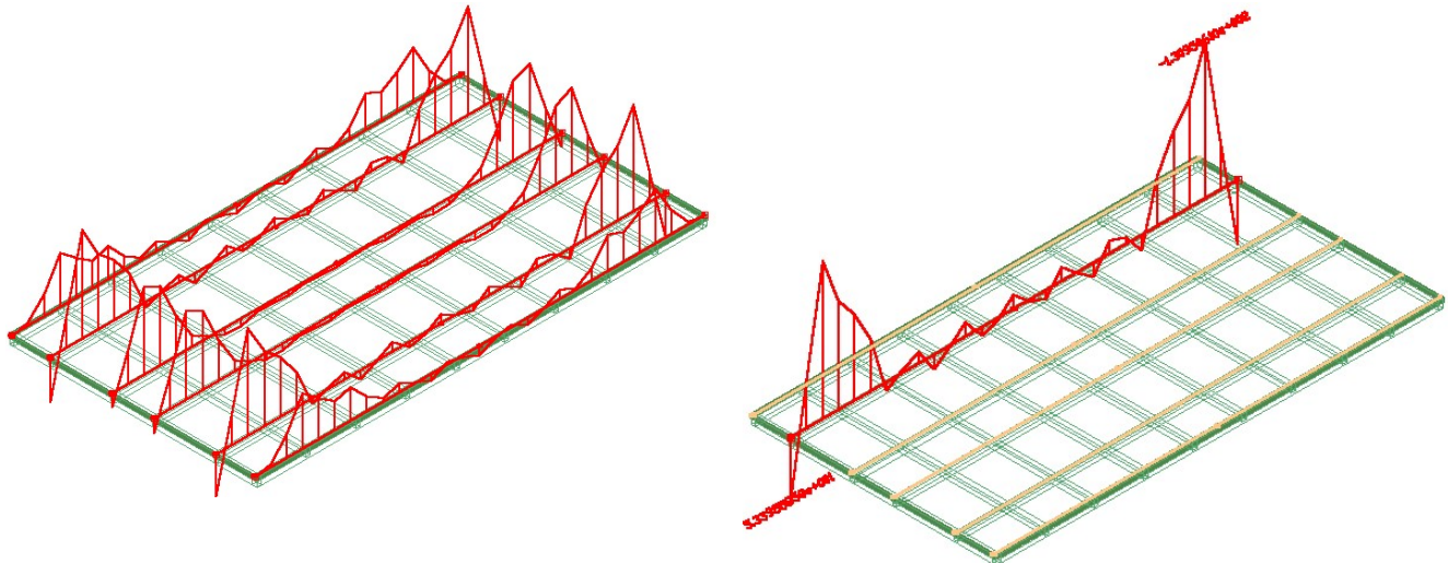
(a) Moments for long direction Design Strips
