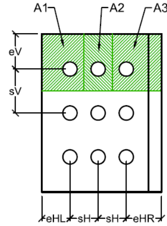
Clip Angle (Multiple rows of bolts)
