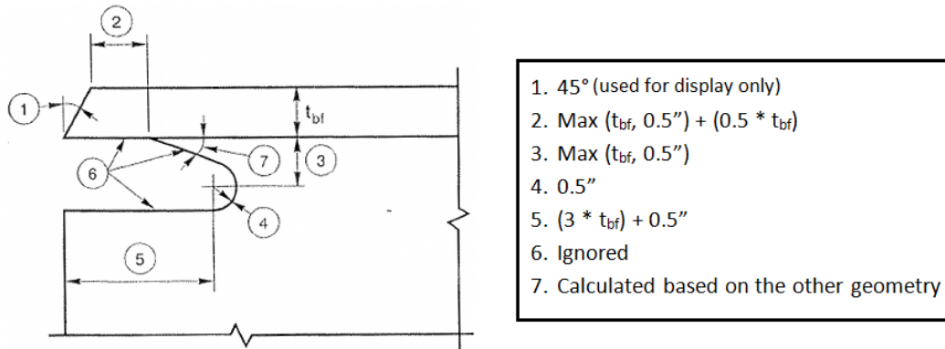
AWS D1.8/D1.8M Figure 6.2
